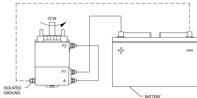
FIGURE-2 MOTOR-COUNTER CLOCKWISE ROTATION
